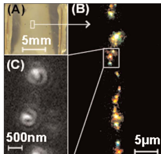
Shown here is a (A) discolored silver oxide region between copper electrodes on a glass substrate in a vacuum, DC potentials of 9 volts were applied across the film; (B) multi-colored electroluminescence from single silver molecules occurs within the electrically discolored region. (C) These features exhibit dipole emission patterns and blinking dynamics (not shown) characteristics of single-molecule behavior.
